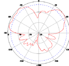
E Plane
