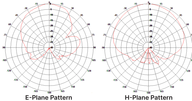
Frequency 5500 MHz
