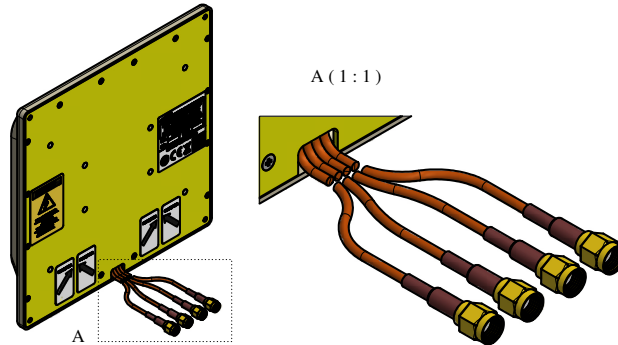
Frequency 2450 MHz
