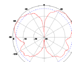
E Plane
