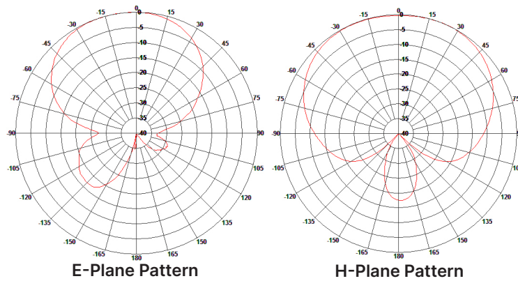
Frequency 5500 MHz
